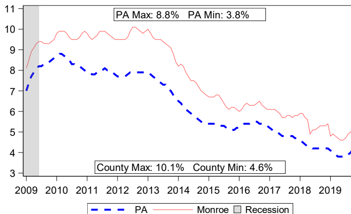
Unemployment Rate, Jan 2009 to Nov 2019
